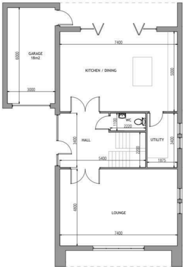
GROUND FLOOR GIA - 98.8m2 (exc garage)
